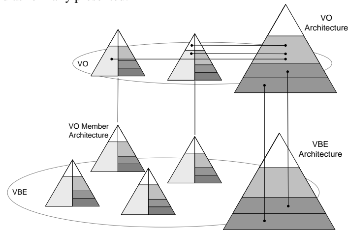
Figure 3 Virtual Organization architecture development. The two lowest architecture domains are shared with the VBE; the service architecture domain integrates services from VO members
