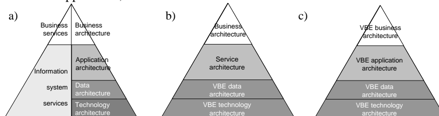
Figure 2: Architecture domains: a) TOGAF b) VO c) VBE
