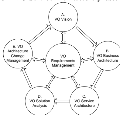
Figure 3. Architecture Development Method for Virtual Organization (ADM4VO)
